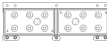
2 Cell (17–33 plates)
