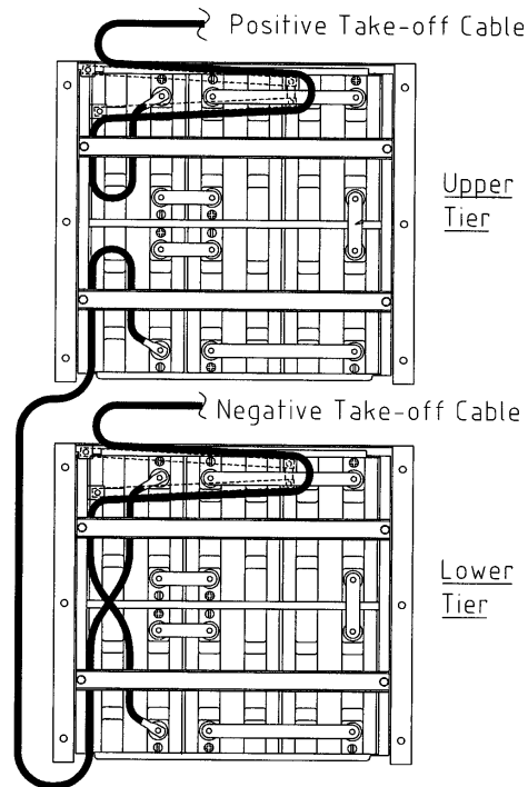
48V, 150AH BATTERY LAYOUT
