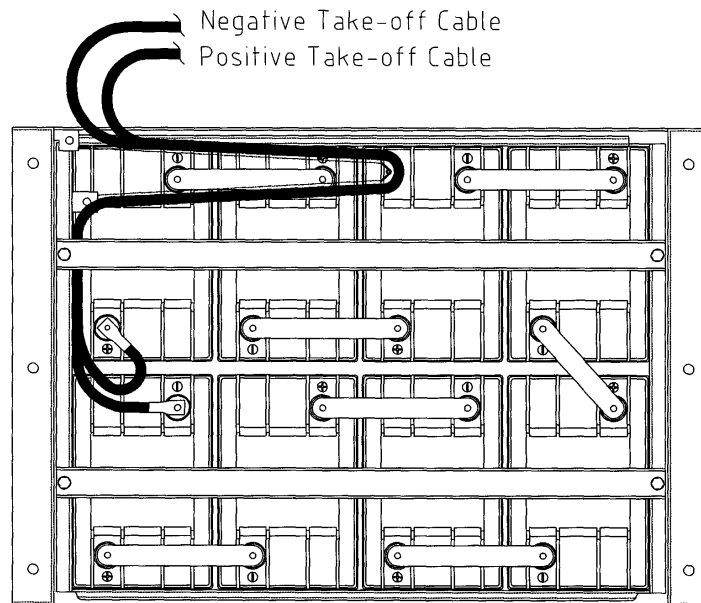
48V, 125AH BATTERY LAYOUT
