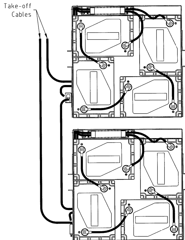
48V, 160AH BATTERY LAYOUT
